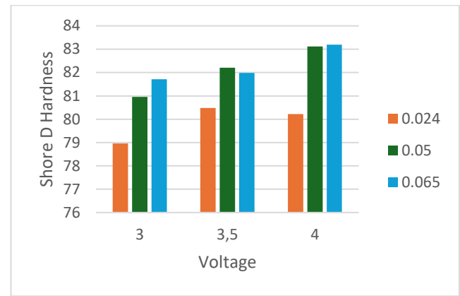
Figure 5. Hardness Value
