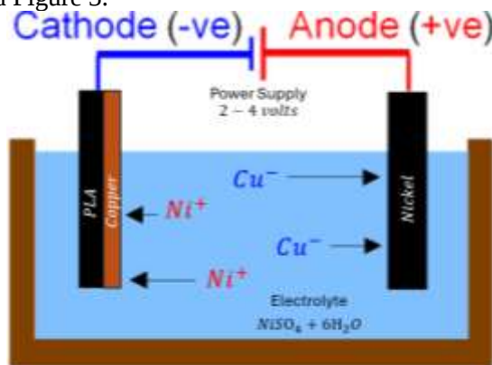
Figure 2. Electroplating Schematic Diagram
