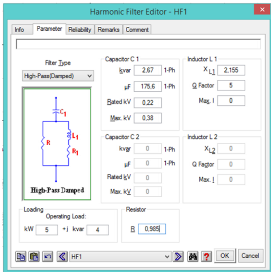
Gambar 3. Harmonik filter editor FL-1
