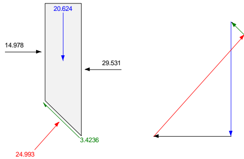
Slice 9 - Bishop Method
