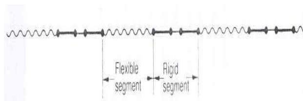
Figure 1. Primary structure of polyurethanes (Uhlig, 1999).
