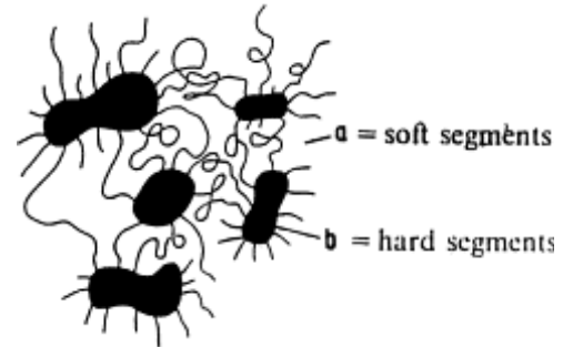
Figure 3. Hard Segments and Soft Segments of Thermoplastic Polyurethanes (Oertel, 1985)
