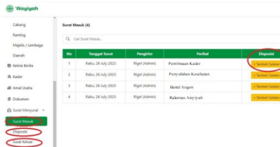
Gambar 5. E-Surat
