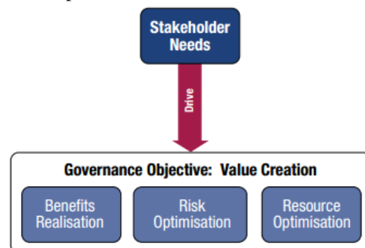
Gambar 3.1 Kebutuhan Stakeholder
