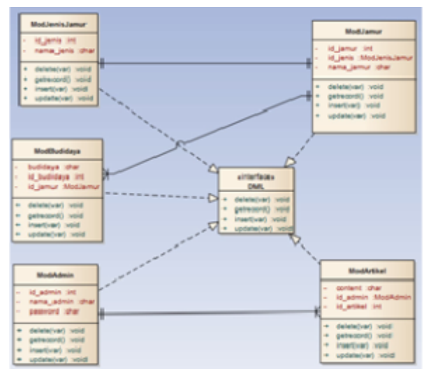
Gambar 3 Class diagram
