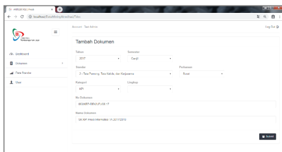
Gambar 9. Form Input
