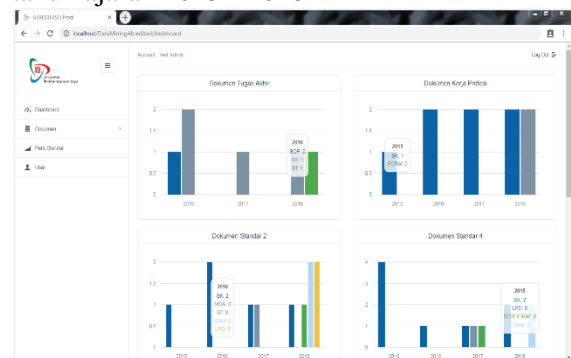
Gambar 10. Tampilan Dashboard
