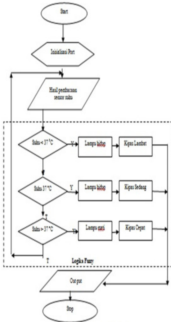
Gambar 7. Flowchart Sistem
