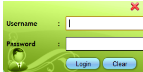
Gambar 4. Form login
