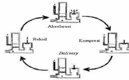
Gambar 1. Siklus kerja pompa hydraulic ram pump .
