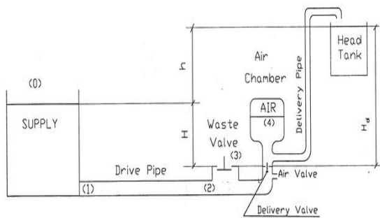
Gambar 2. Skema instalasi pompa hydraulic ram pump (Taye, 1998)
