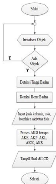
Gambar. 3.2 Flowchart Program
